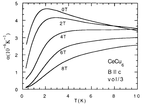
Fig. 2. Coefficient of volume expansion of \text{CeCu}_6 divided by 3 ( \alpha_v/3 ) vs temperature at fields ( B \parallel c ) as indicated.
