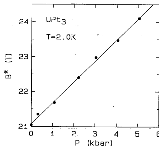
FIG. 2. Pressure variation of the metamagnetic threshold field B^* of UPt_3 at T=2.0 \text{ K} . B^* increases at a constant rate of 0.60 \text{ T/kbar} (solid line).
