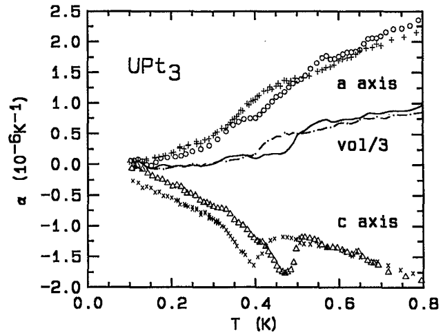
FIG. 2. Coefficient of linear thermal expansion of \text{UPt}_3 vs temperature along the a and c axes for sample 1 ( +, x ) and sample 2 ( \circ, \Delta ). The dashed and solid lines correspond to \alpha_v/3 (for samples 1 and 2, respectively).
