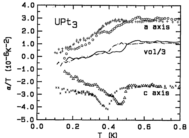
FIG. 3. Coefficient of linear thermal expansion of \text{UPt}_3 in a plot of \alpha/T vs T , along the a and c axes for sample 1 ( +, x ) and sample 2 ( \circ, \Delta ). The dashed and solid lines correspond to \alpha_v/3 (for samples 1 and 2, respectively).
