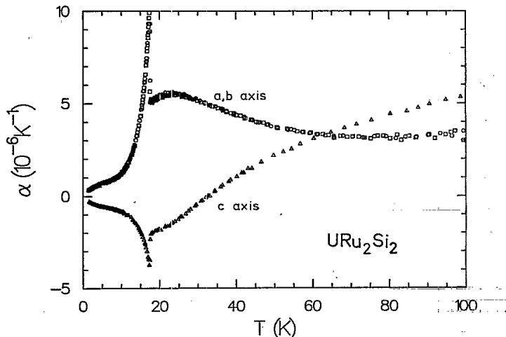
FIG. 1. The thermal-expansion coefficient \alpha (=L^{-1}\Delta L/\Delta T) along the three crystallographic axes of the tetragonal compound URu_2Si_2 ; a axis ( \circ ), b axis ( \square ), c axis ( \Delta ).
