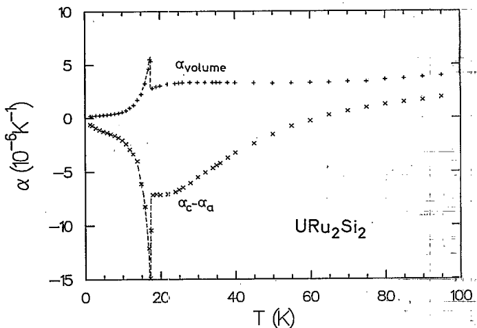
FIG. 2. The volume thermal-expansion coefficient \alpha_v = (\alpha_a + \alpha_b + \alpha_c)/3 , and the relative temperature dependence of the c/a ratio \alpha_r = \alpha_c - \alpha_a , as determined from the data of Fig. 1; \alpha_v (+), \alpha_r (x).
