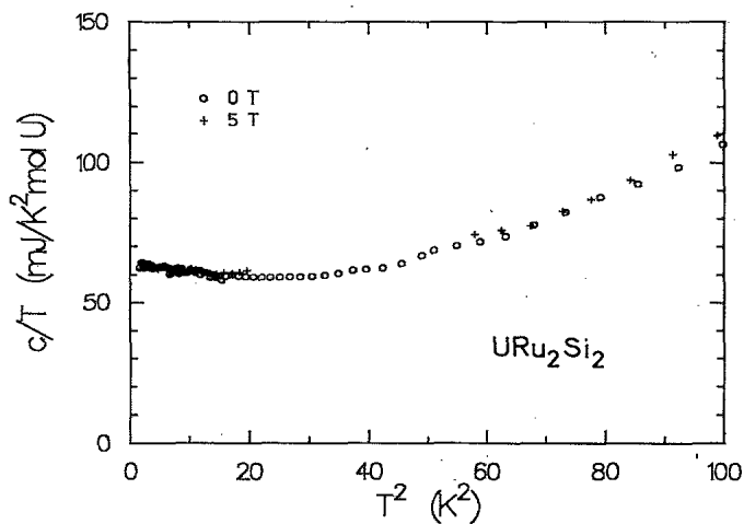
FIG. 5. The specific heat of URu 2 Si 2 plotted as c/T vs T^2 in zero field (○) and in an applied field of 5 T (+).
