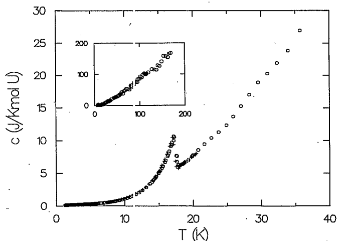
FIG. 4. The specific heat of URu_2Si_2 as a function of temperature in zero field ( \circ ) and in 5 T (+). The inset shows the specific heat up to 170 K.
