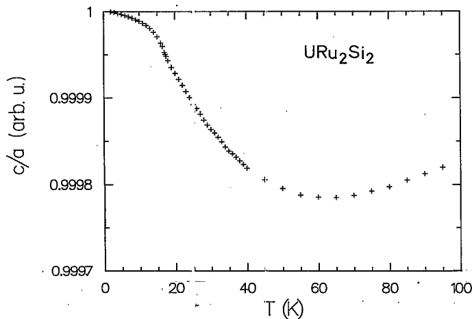
FIG. 3. The c/a ratio of URu_2Si_2 normalized to 1 at 1.4 K, as a function of temperature
