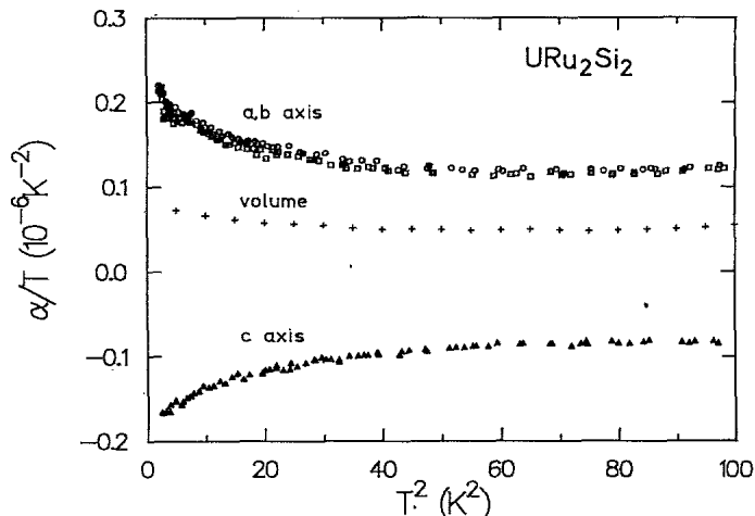
FIG. 6. The thermal expansion of URu 2 Si 2 plotted as \alpha_i/T vs T^2 ; \alpha_a (○), \alpha_b (□), \alpha_c (△), \alpha_v (+).
